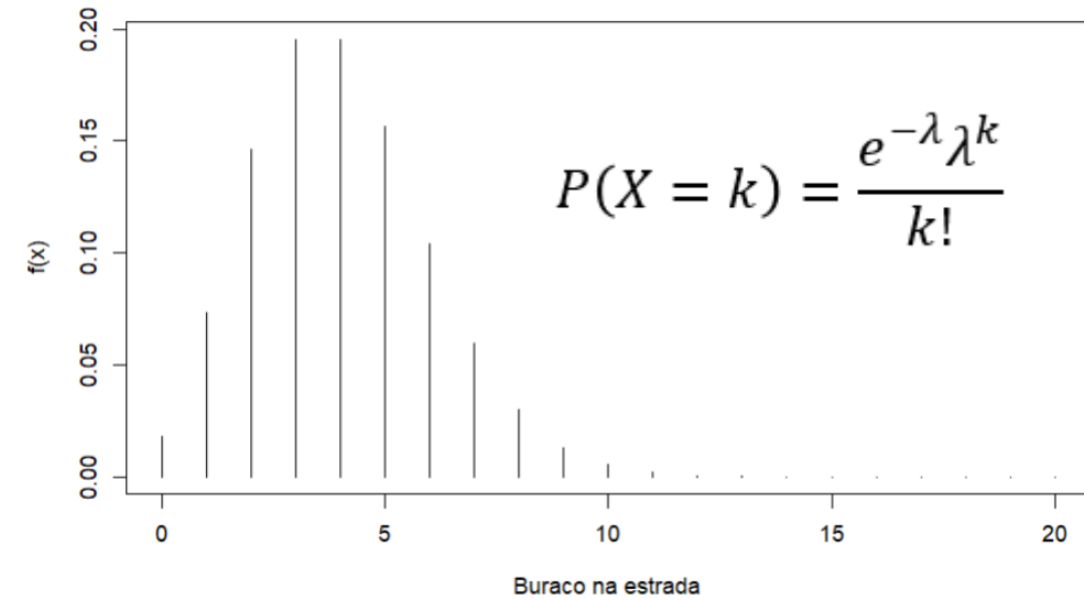
Poisson (taxa = 4 / Km)
