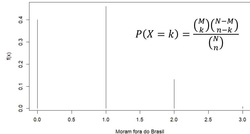
Hypergeométrica (Moram fora = 5, Moram Brasil = 15, n = 3)
